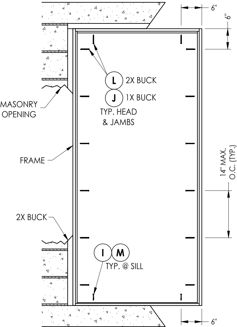
FRAME ANCHORING
