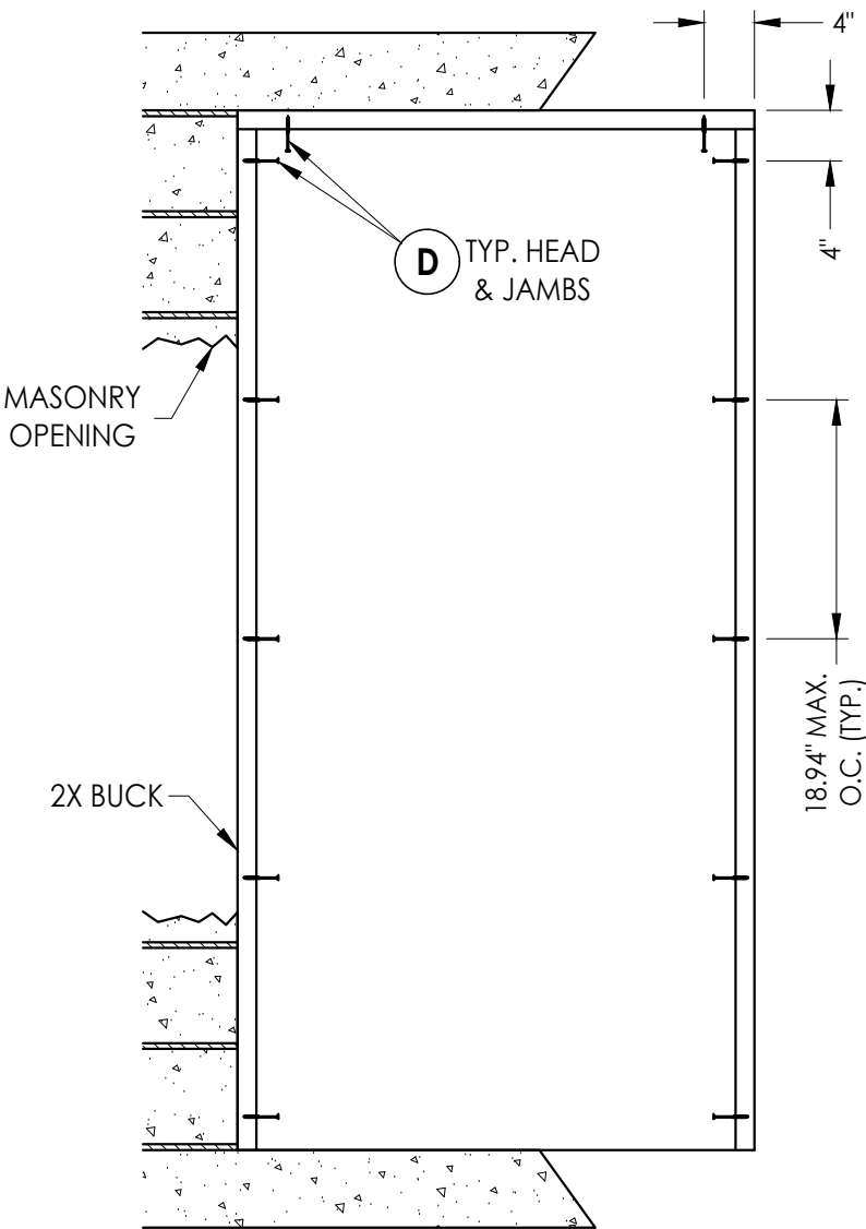
BUCK ANCHORING
